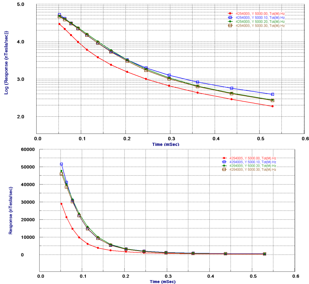
Fig. 39: Focus on early off-time data from the previous figure
