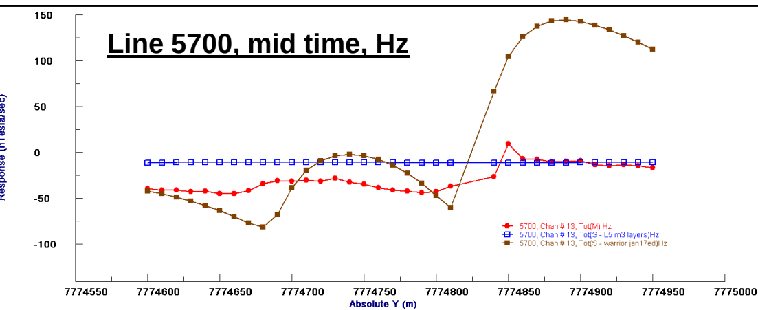
Figure 11: Profile response along Line 5700E (east line) for Loop 5, comparing the measured response with the simulated response of the background model and the 2010 plate model derived from the larger loop data. Early time (Ch. 6) and mid time (Ch. 13) for Hz are shown.
