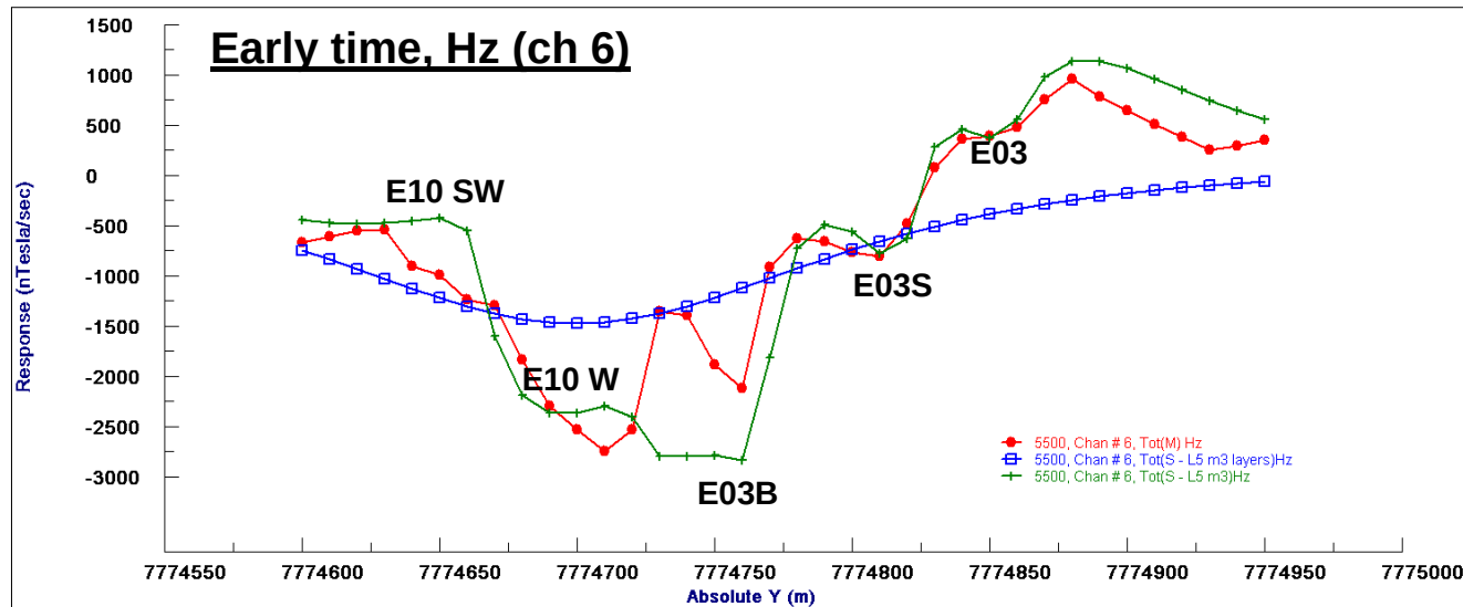
Fig. 12: Comparison of the Loop 5 model response vs. the measured data on Line 5500E for Hz and Hx, early time.
