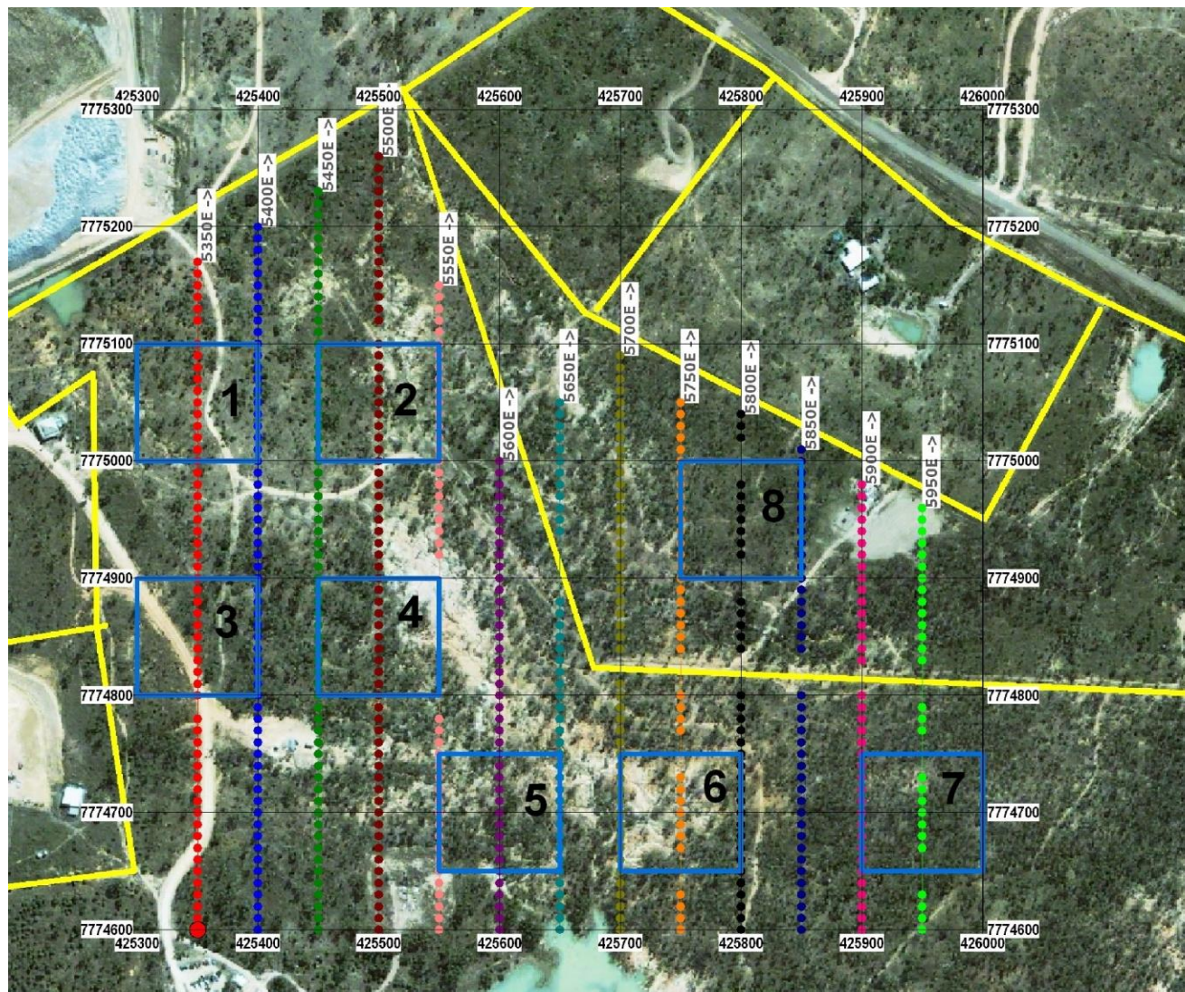
Figure 9: Planned loops and lines for Summer 2011 ground TEM survey.
