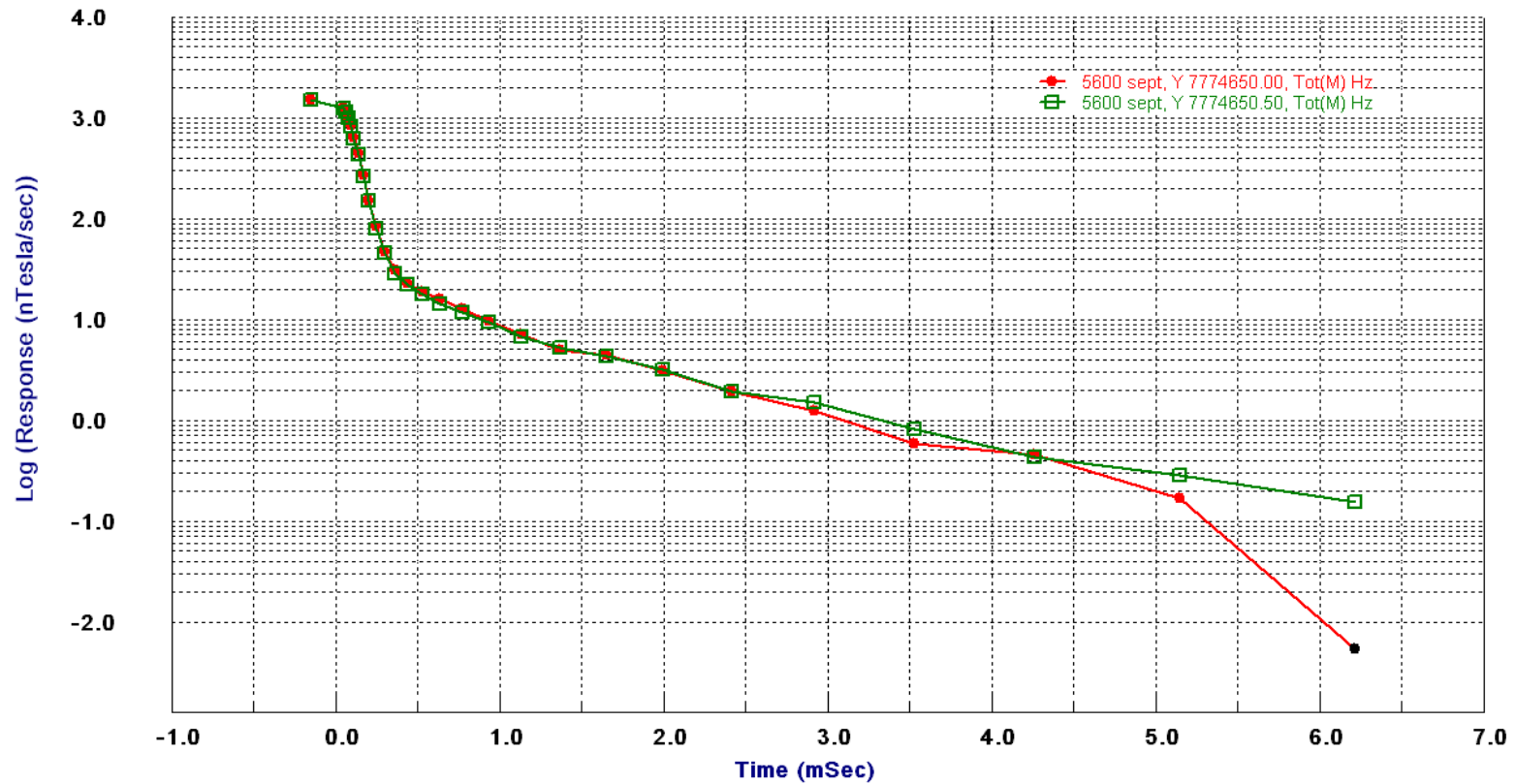
Figure 53: Comparison Khumsup data (Hz) at 7774650N on Line 5600E on two different days.
